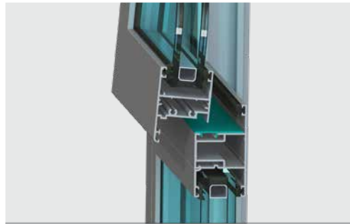
Kleenline™ – Sash window frame platform cover
