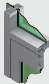
Example of Shop Front 106mm with commercial door
